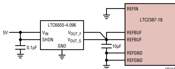
Figure 9. Overdriving REFBUF Using the LTC6655-4.096
